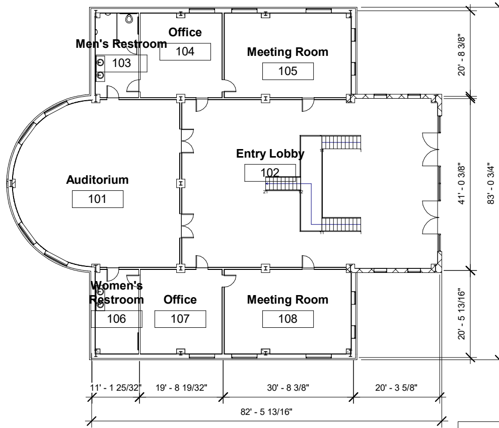
① Level 1 Floor Plan 1/16" = 1'-0"
